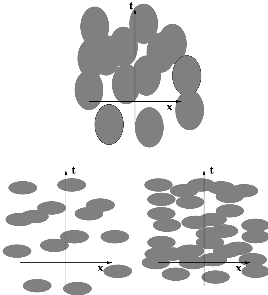
Figure 1: Top: Support of unscaled Poisson blobs. Left hand side: Support of Poisson blobs distributed according to a fixed intensity rescaling. Right hand side: Support of Poisson blobs distributed according to a diffusive (D) rescaling.
