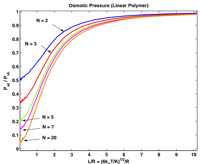
FIG. 4: Correction Factor for a Linear Polymer Confined in a Spherical Chamber. The classical van't Hoff's Law for N free monomers is P_{vh} = Nk_B T / \frac{4}{3}\pi R^3 . For stretching an individual bond between monomers, we let L = (6k_B T/K)^{1/2} denote the length at which the bond energy becomes 3k_B T .
